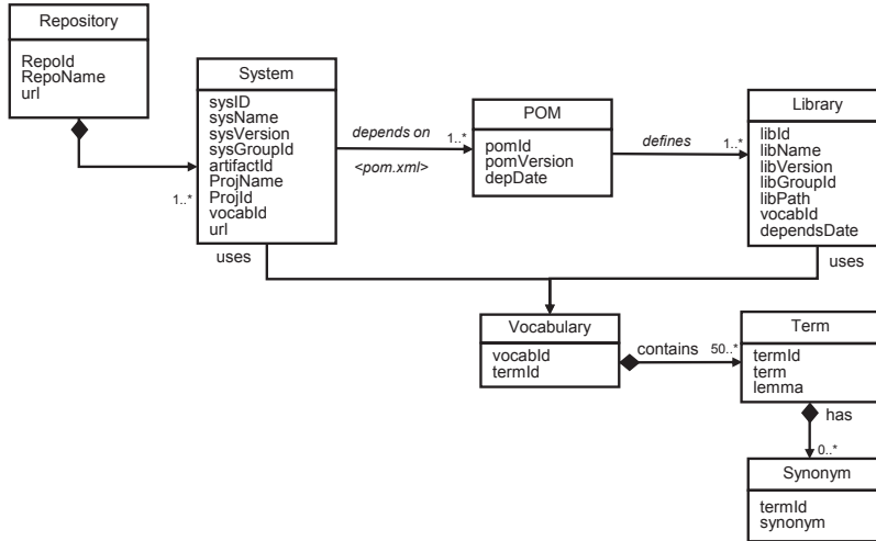
Figure 4: The data model of the collected dataset.
