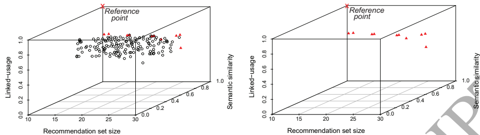
(a) Last iteration solutions (depicted by the circles) and Pareto surface (depicted by the red triangles) obtained by NSGA-II. (b) Pareto surface (depicted by the triangles) obtained by NSGA-II.
