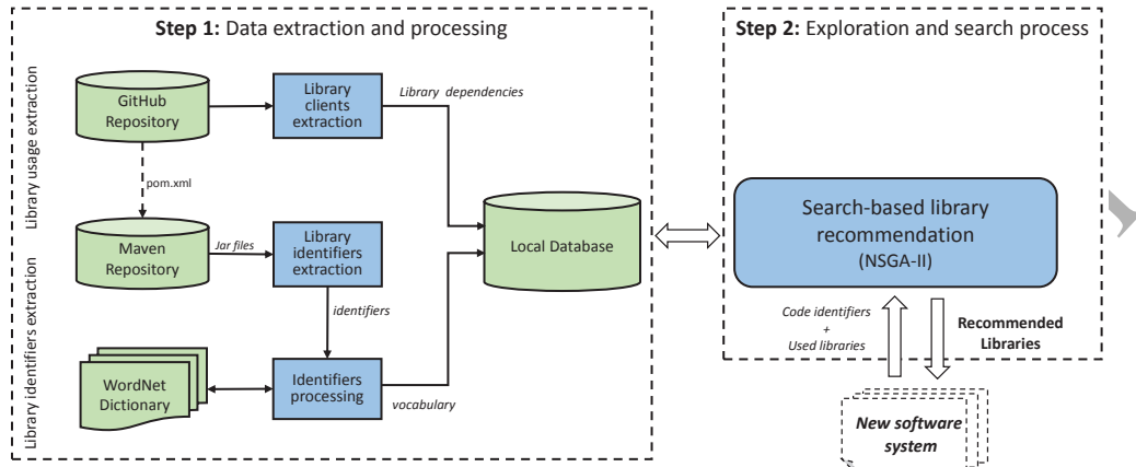
Figure 2: Our search-based library recommendation framework LibFinder .
