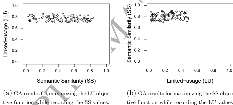
Figure 9: Relation study between the Linked Usage (LU) and Semantic Similarity (SS) objective functions.
