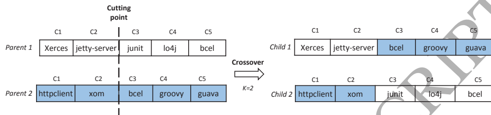
Figure 6: Crossover operator.
