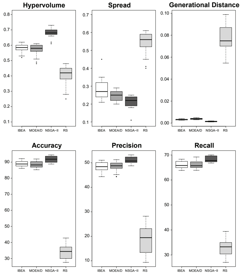
Figure 8: Boxplots for the Hypervolume, Spread, Generational distance, accuracy@10, precision@10 and recall@10 performance indicators for NSGA-II, IBEA, MOEA/D and RS.
