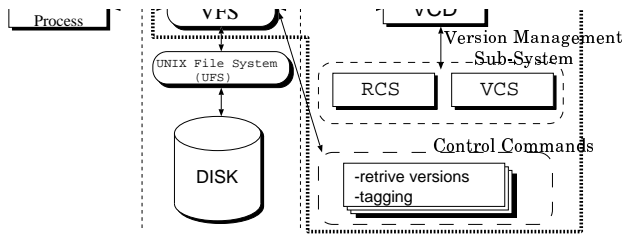
Figure 1: Architecture of Moraine
