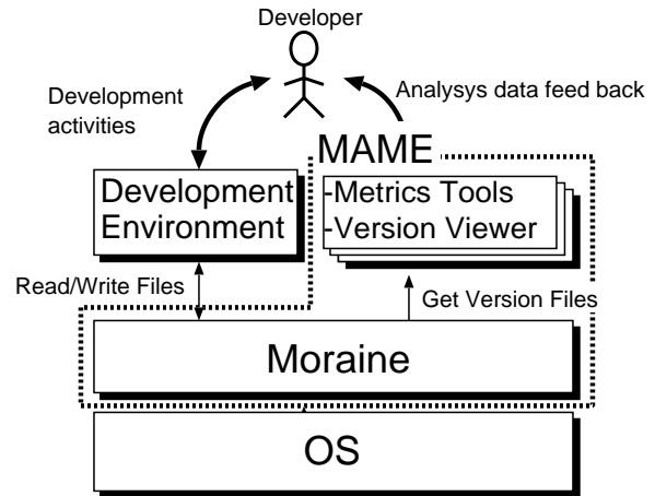
Figure 5: MAME architecture
