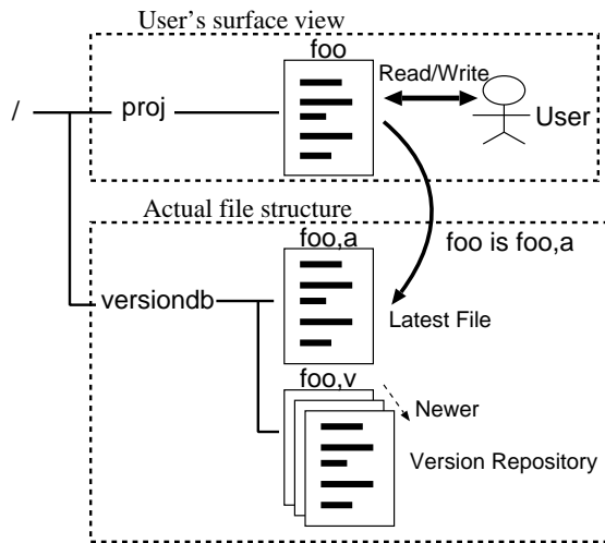
Figure 2: Mapping files between VCFS and actual file system
