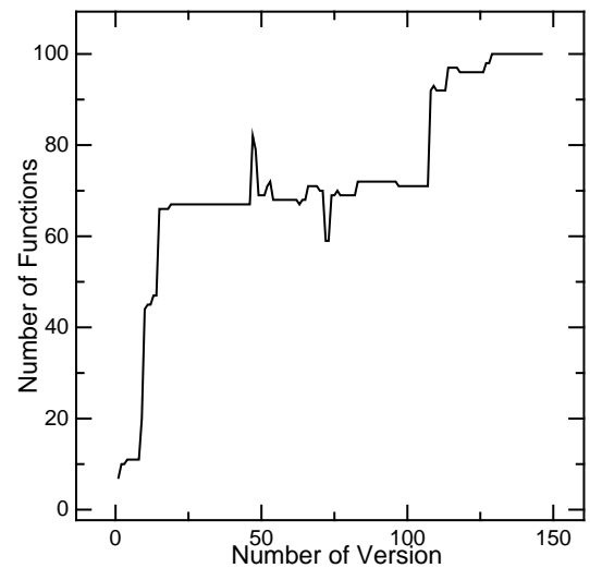
Figure 9: Changes of Number of Functions (Student 2)
