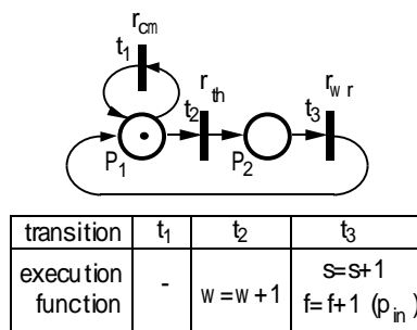
Fig. 4 Activity model
