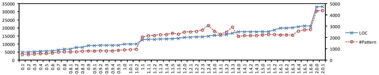
Figure 2. LOC and the number of patterns of dnsjava
