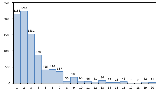
Figure 5. Life-span of patterns in JmDNS
