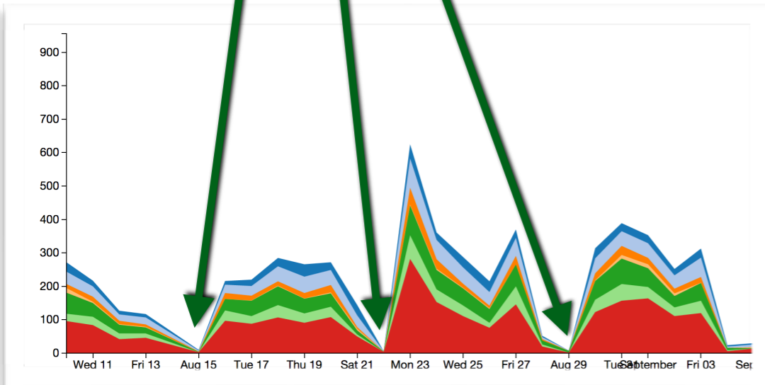
Activity Statistic
