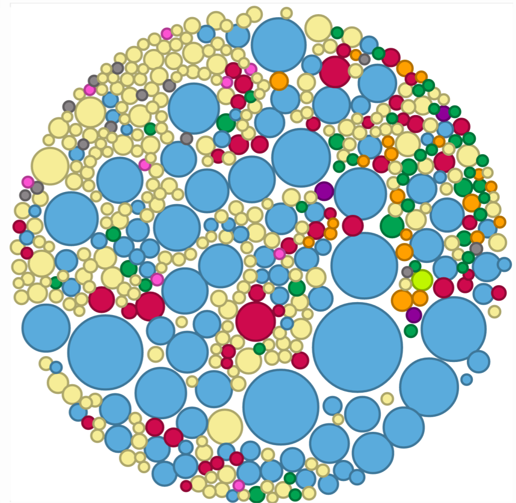
Contributor Activities
