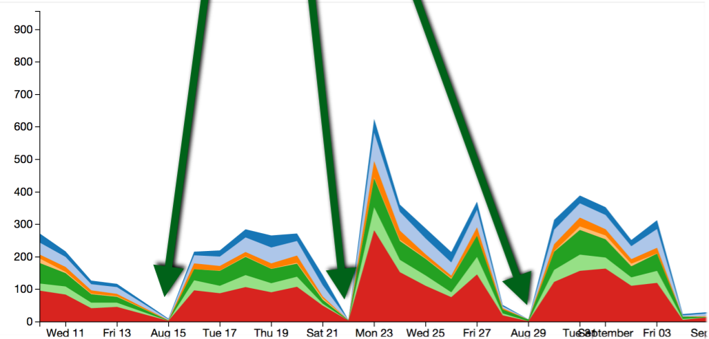
Activity Statistic
