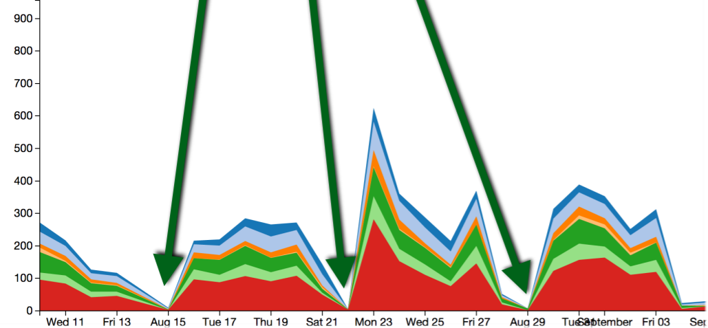
Activity Statistic
