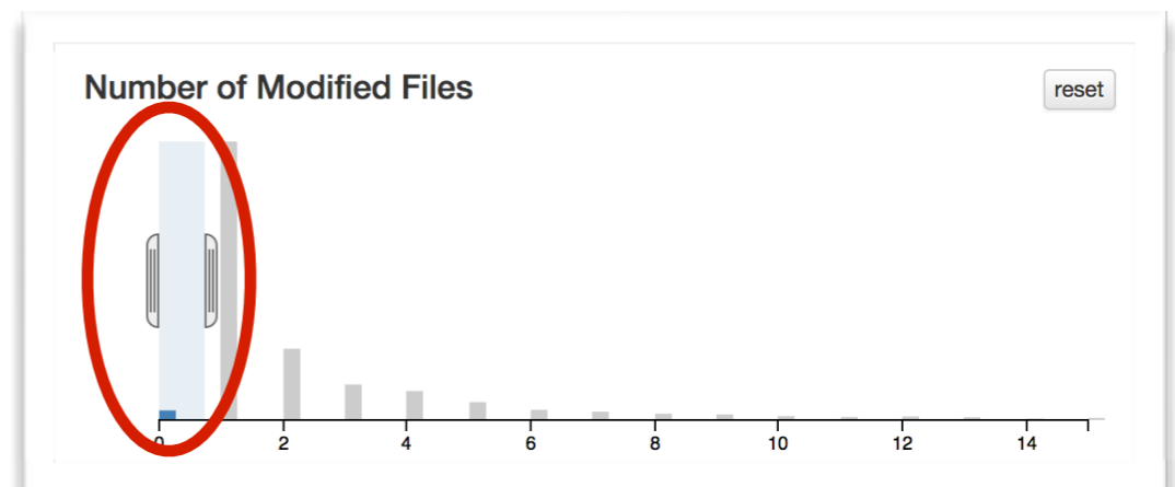
Review Statistic
