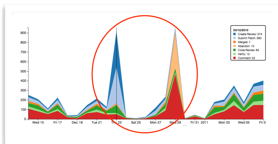
Activity Statistic
