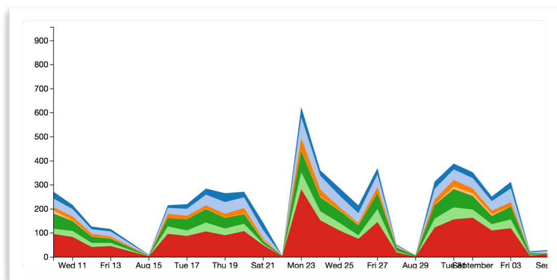
Activity Statistic
