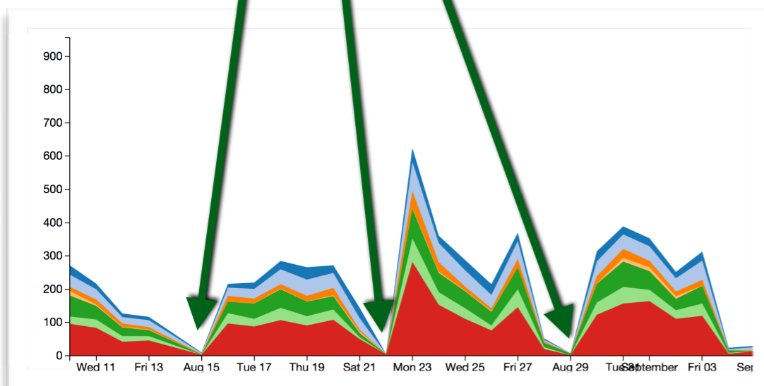
Activity Statistic
