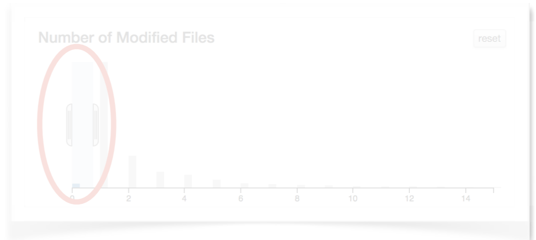
Review Statistic
