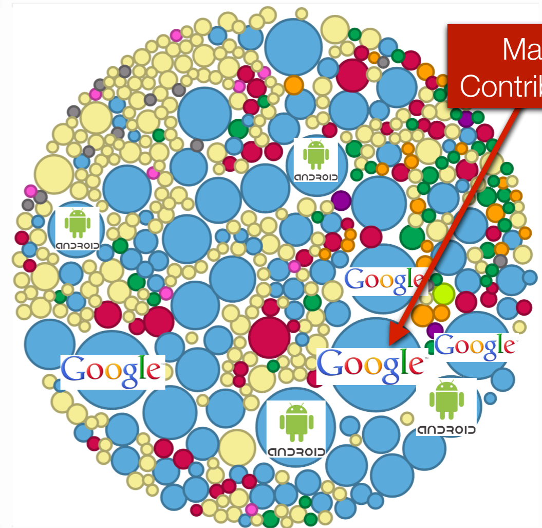
Contributor Activities
