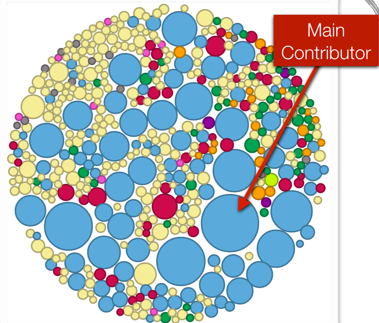
Contributor Activities
