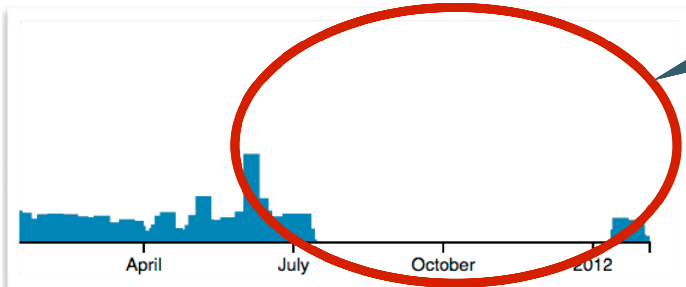
Review Statistic
