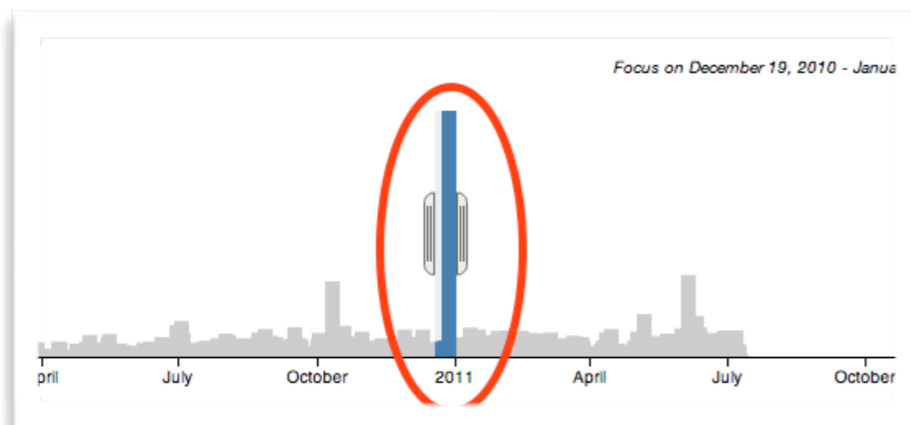
Review Statistic
