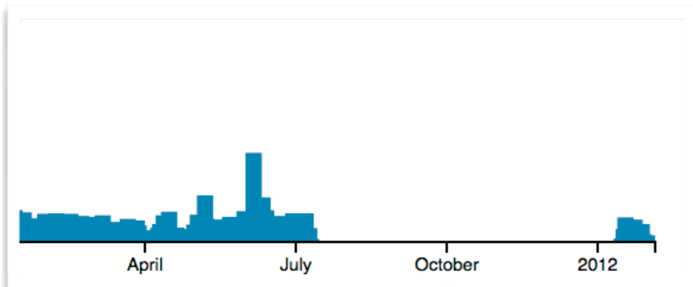
Review Statistic
