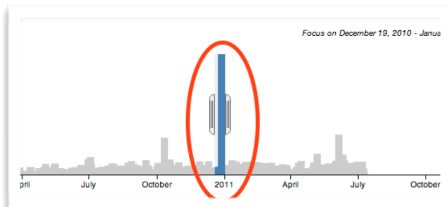
Review Statistic
