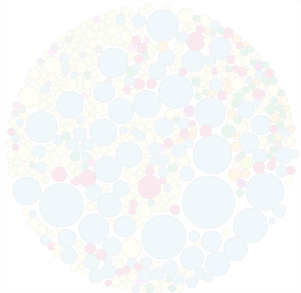
Contributor Activities
