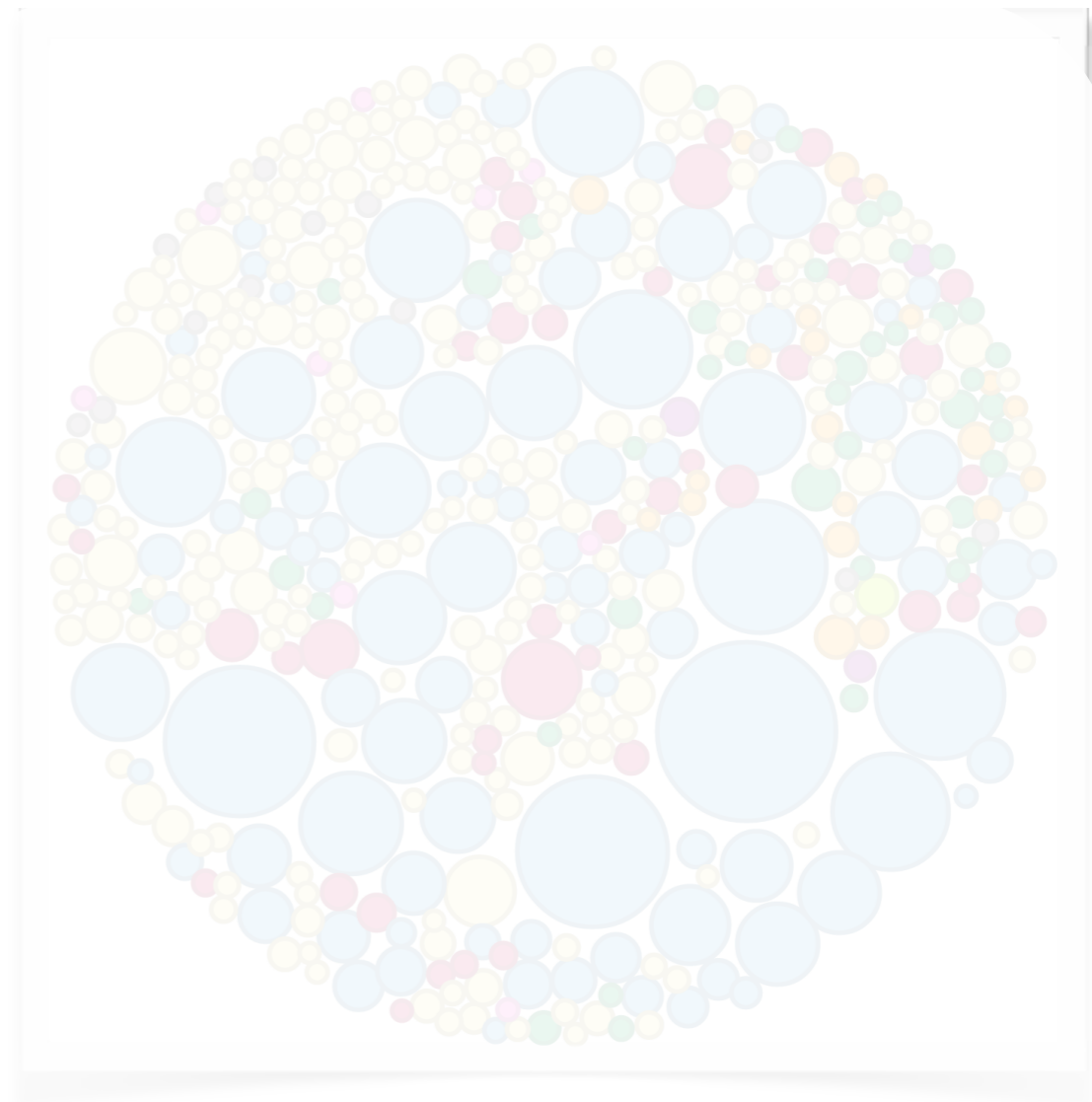
Contributor Activities
