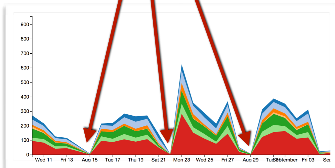
Activity Statistic
