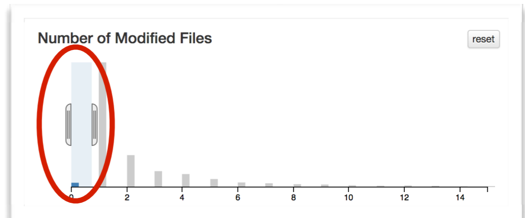
Review Statistic
