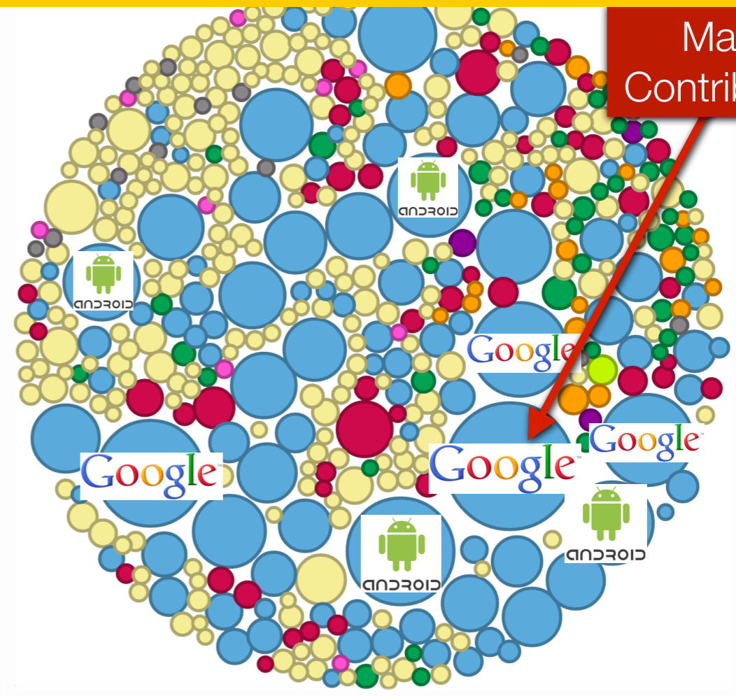
Contributor Activities
