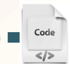
Code change
